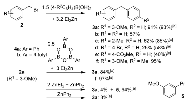
Scheme 1. Selected examples of the arylation of benzyl halides [10] in dioxane at 60 °C for 18 h. [a] 1 H NMR spectroscopic yields.
